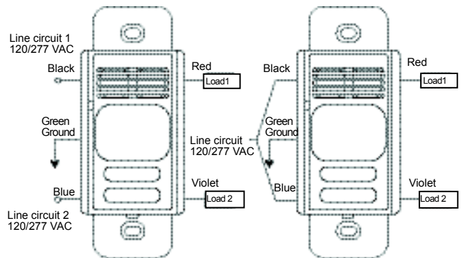
Dual Circuit Sensor (Wired for Dual Circuits)
