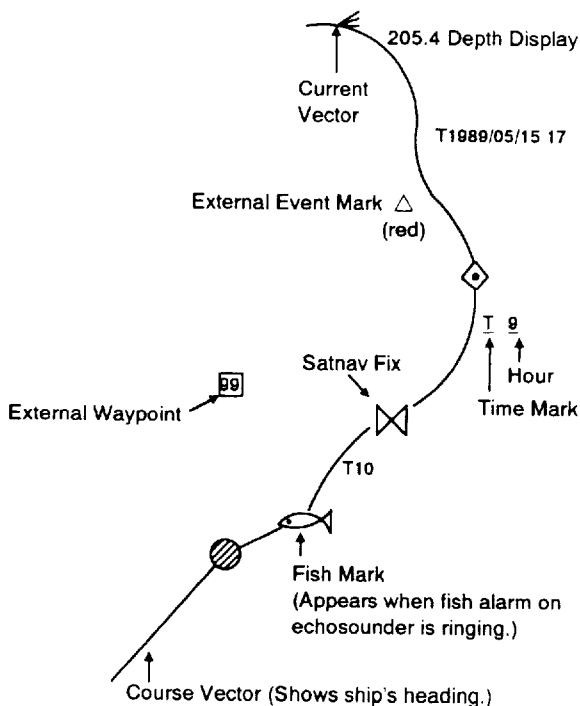
Figure 3-13 Auxiliary marks
