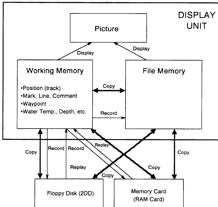
Figure 7-1 Memory configuration
