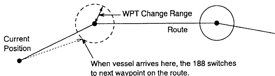
Figure 5-8 Graphic interpretation of waypoint change range
