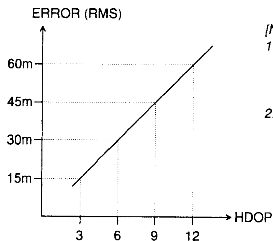
Figure 10-3 HDOP rate and position fix error
