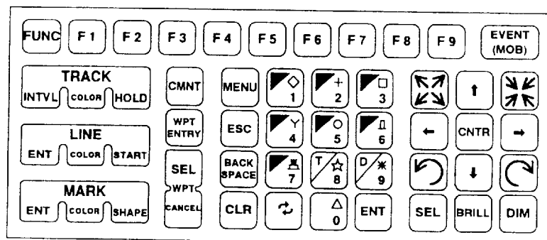
Figure 1-2 Keyboard
