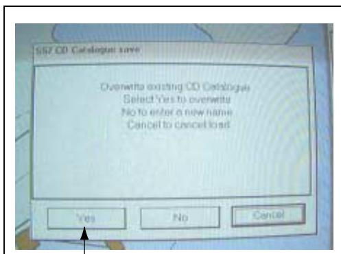
[YES] button
