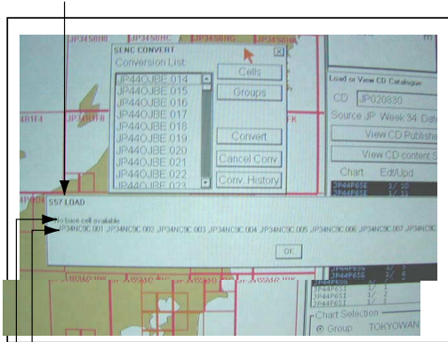
[S57LOAD] window
