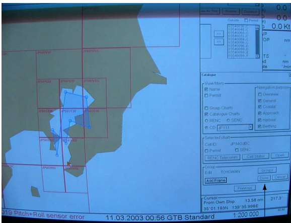
[Done] button
