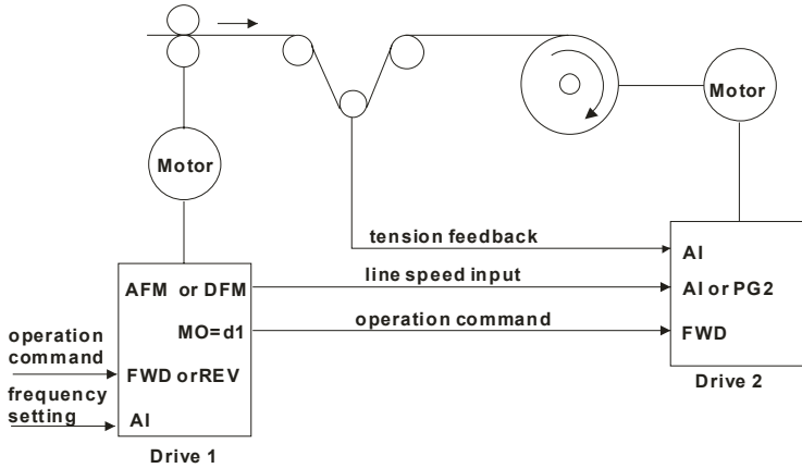
Line speed, speed mode
