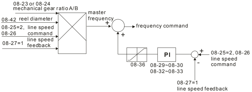
Line speed, speed mode
