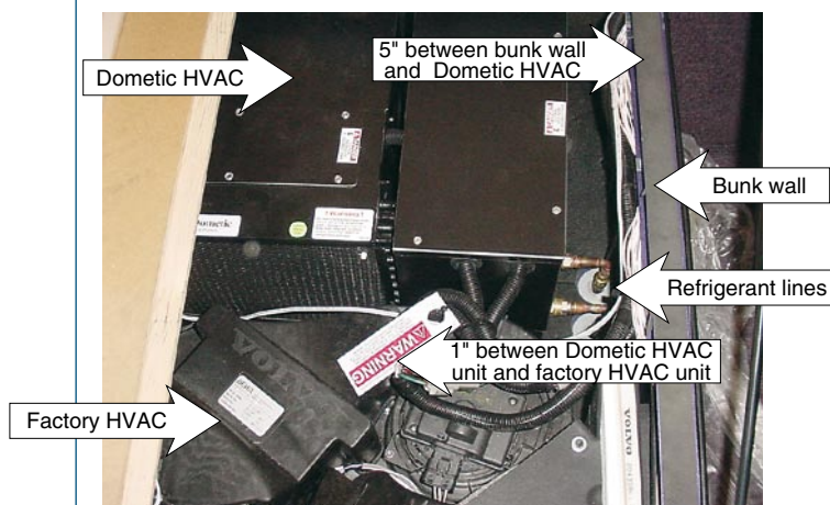
Figure 4 - Installing the CHEB
