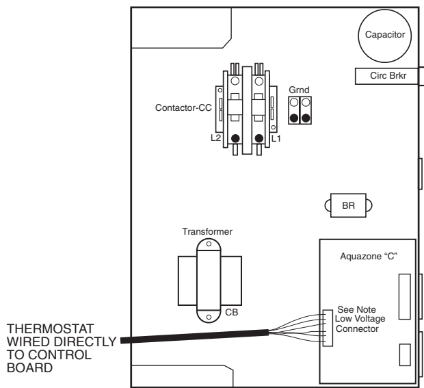
Fig. 17 — Low Voltage Field Wiring
