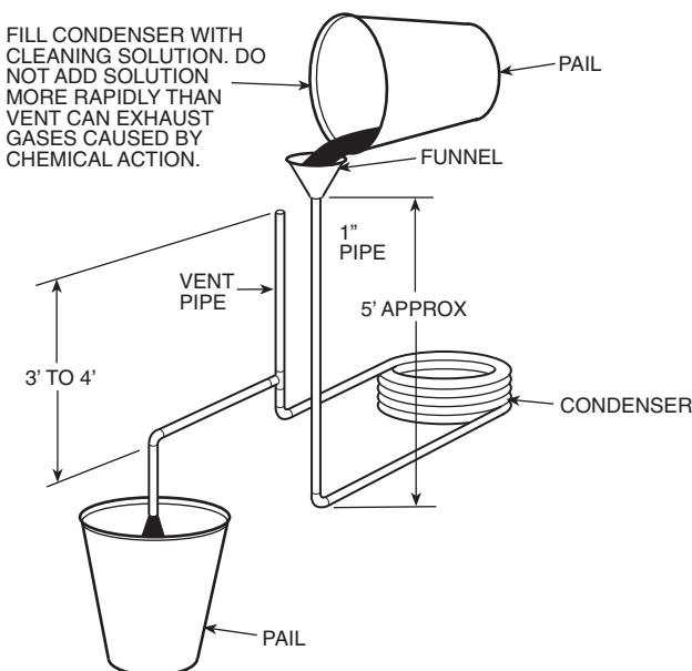
Fig. 23 — Gravity Flow Method
