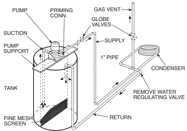
Fig. 24 — Forced Circulation Method
