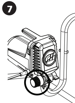
Turn Pressure to HIGH (completely clockwise).
