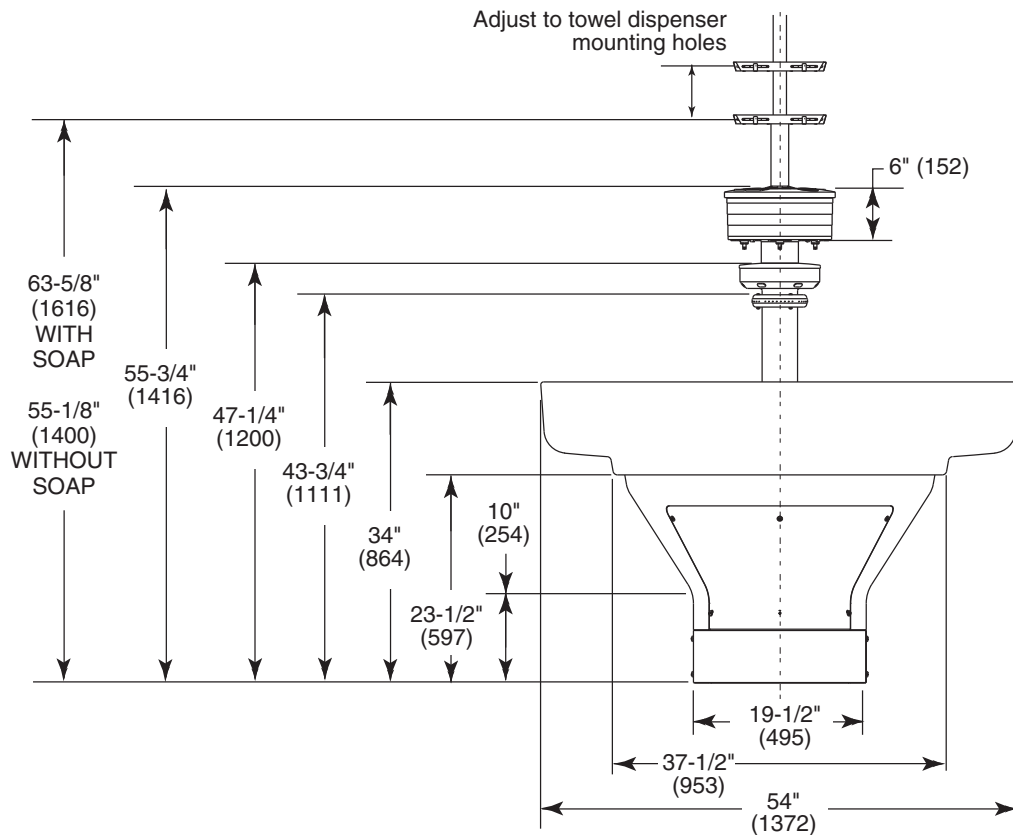
Model WF3208 - 54" Circular with optional accessories
