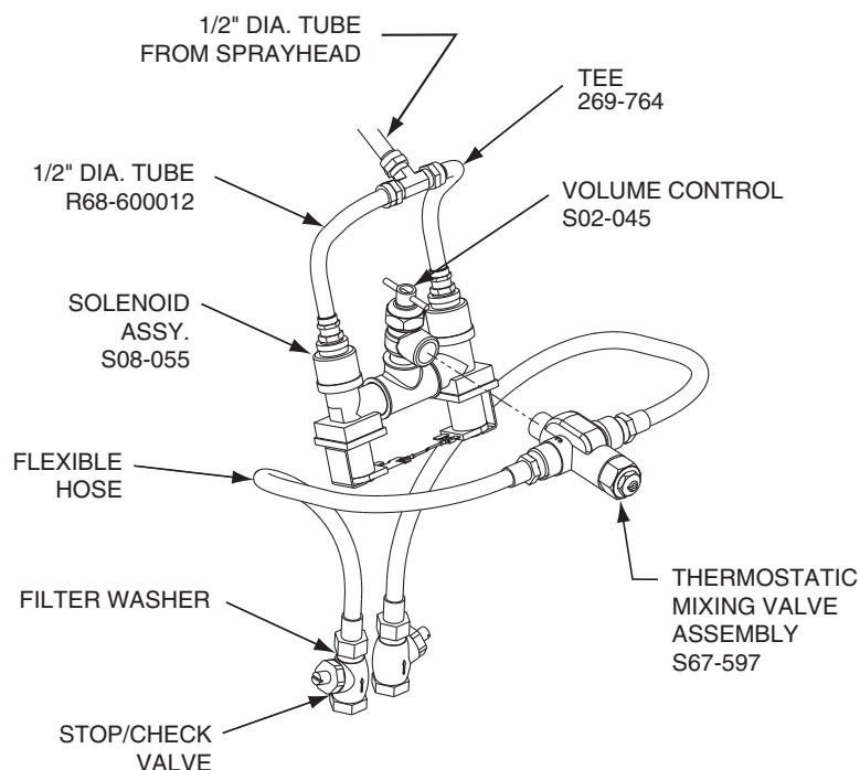
VALVE ASSEMBLY S50-369
