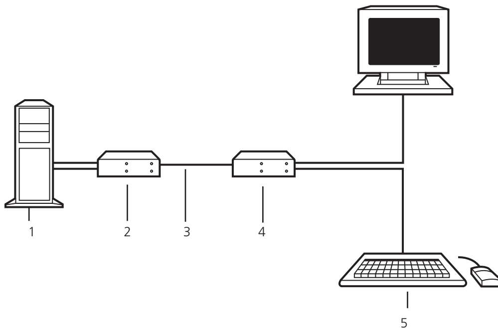
Figure 3-10. DKM Modular Extender (Single-Head).
