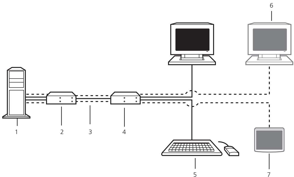
Figure 2-1. System diagram.
