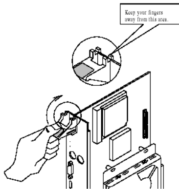
Figure 2.3: Installing a card into the chassis
