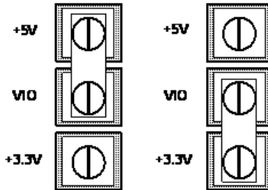
Figure 3.5: V I/O voltage selection
