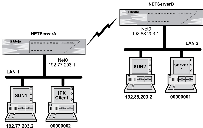
Case Study - LAN to LAN Routing Between Two NETServers
