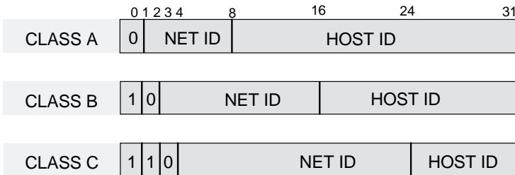
IP Address Classes
