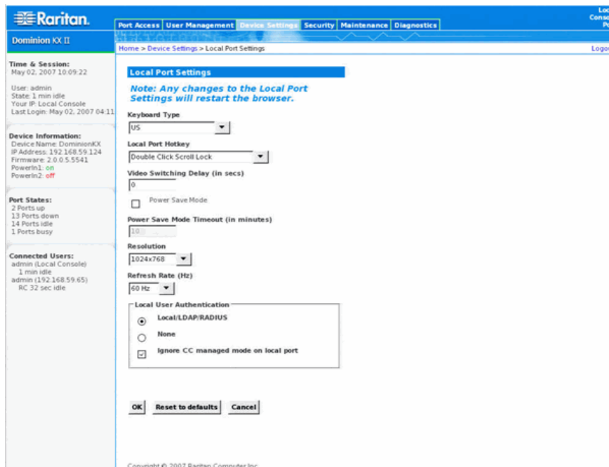
Figure 94: Local Port Settings
