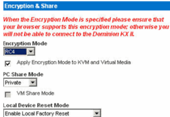
Figure 69: Security Settings (Encryption Mode Warning Message)
