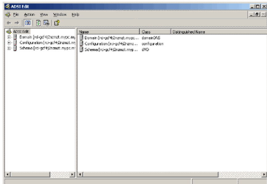
Figure 104: ADSI Edit
