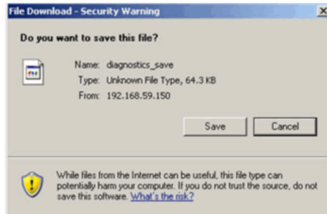
Figure 89: File Download
