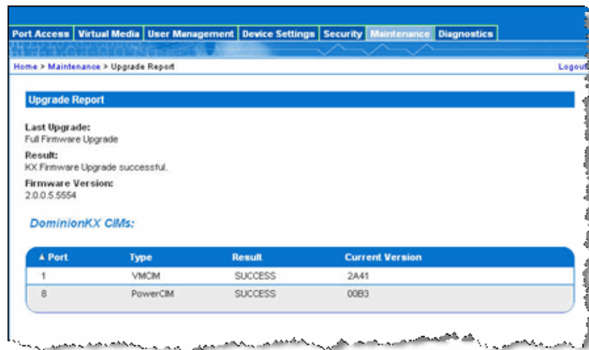
Figure 78: Upgrade Report
