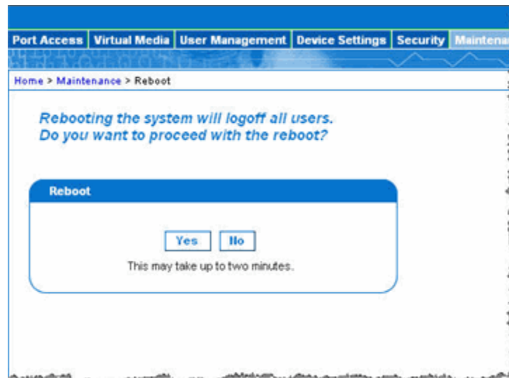
Figure 80: Reboot Confirmation
