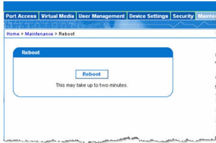
Figure 79: Reboot
