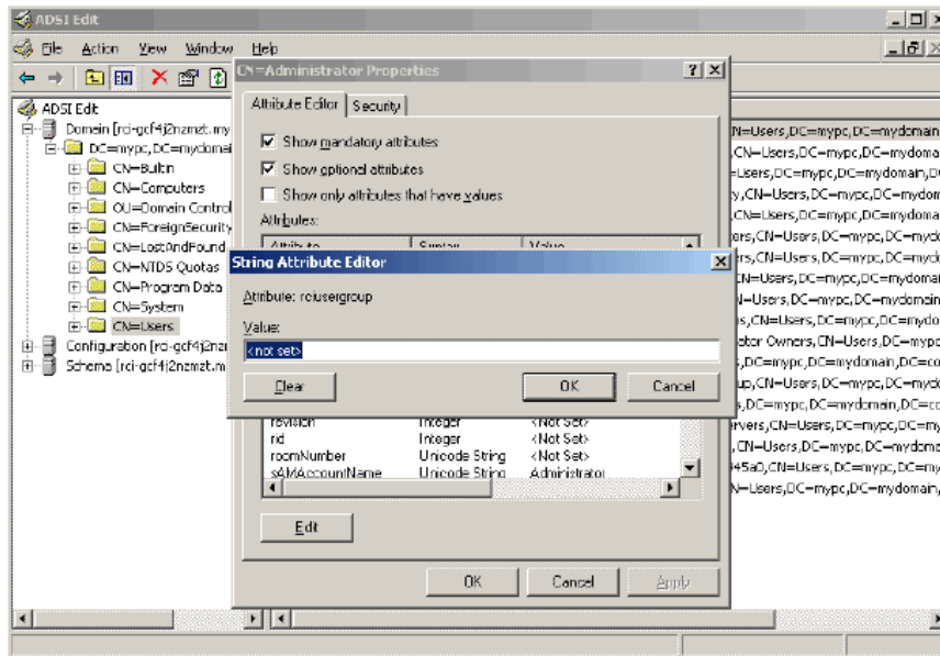
Figure 107: User Properties
