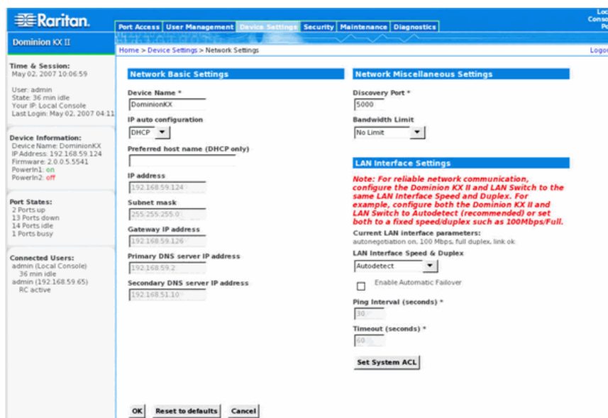
Figure 90: Dominion KX II Local Console
