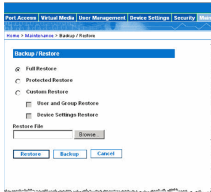
Figure 73: Backup/Restore
