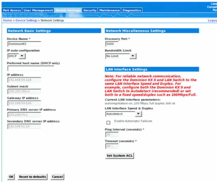
Figure 8: Network Settings
