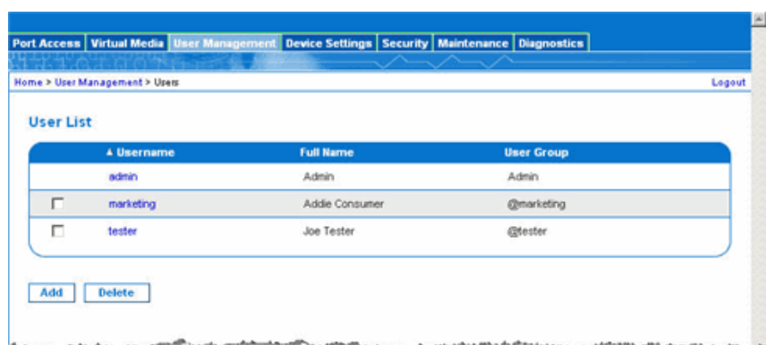
Figure 40: User List
