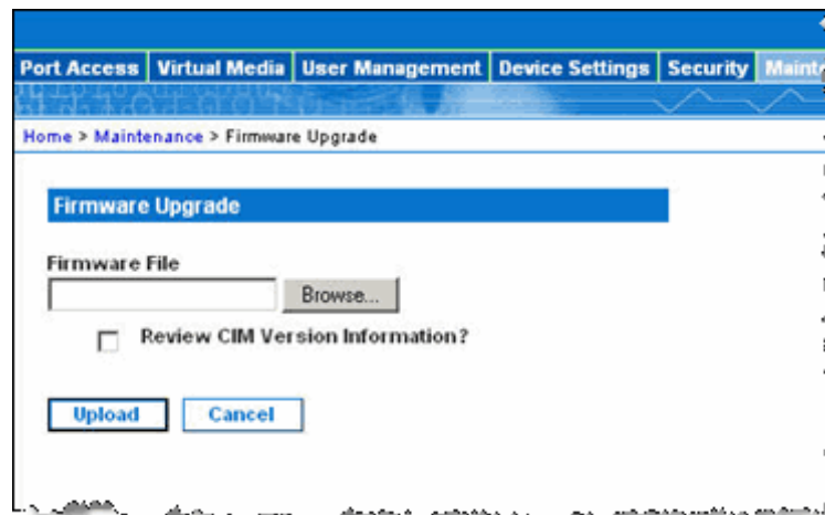
Figure 75: Firmware Upgrade
