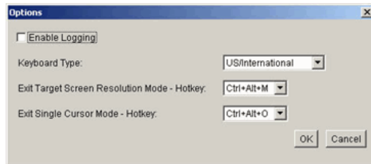
Figure 34: (Tools) Options
