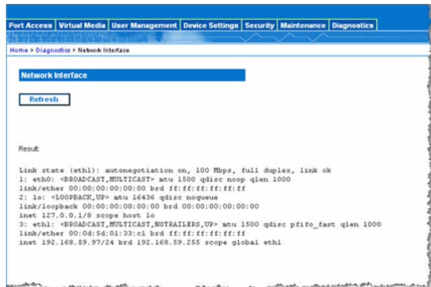
Figure 81: Network Interface
