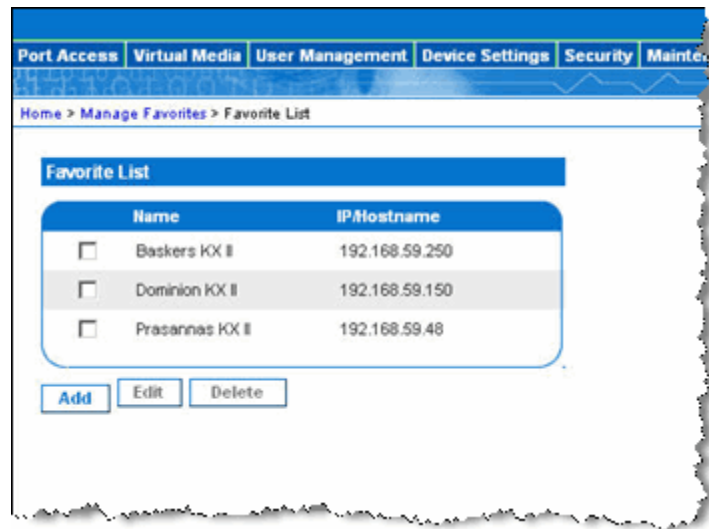
Figure 15: Favorites List
