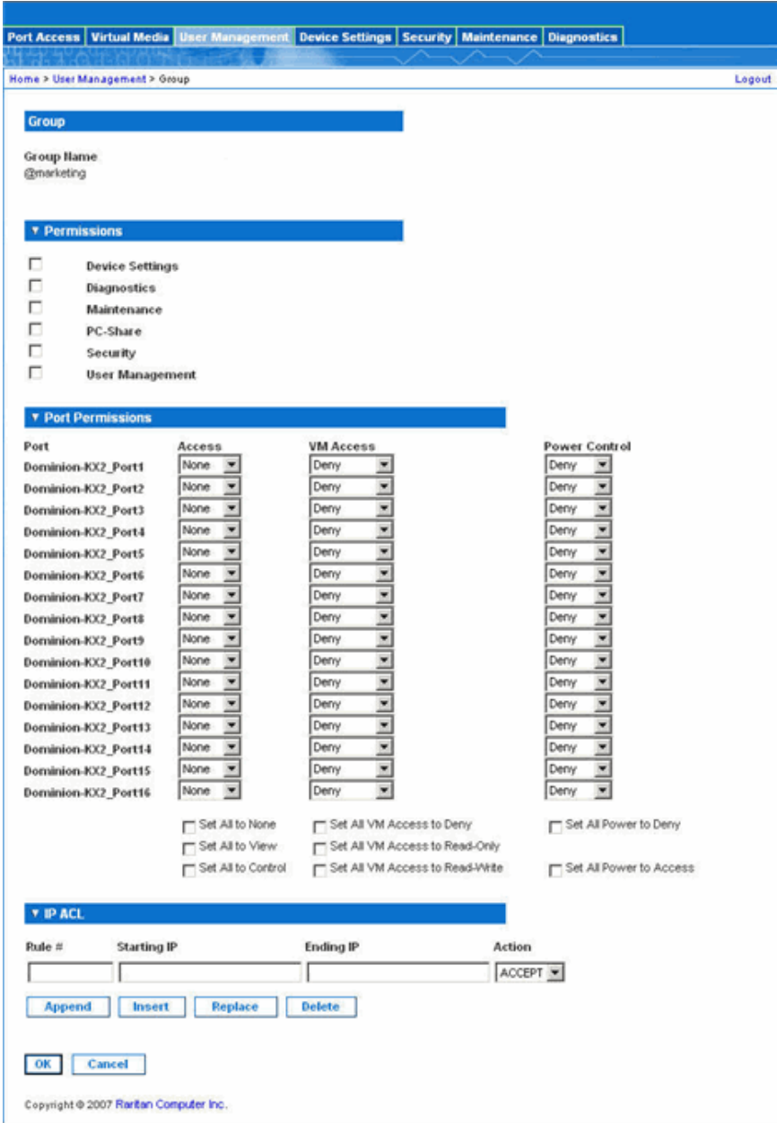
Figure 46: Modify Group
