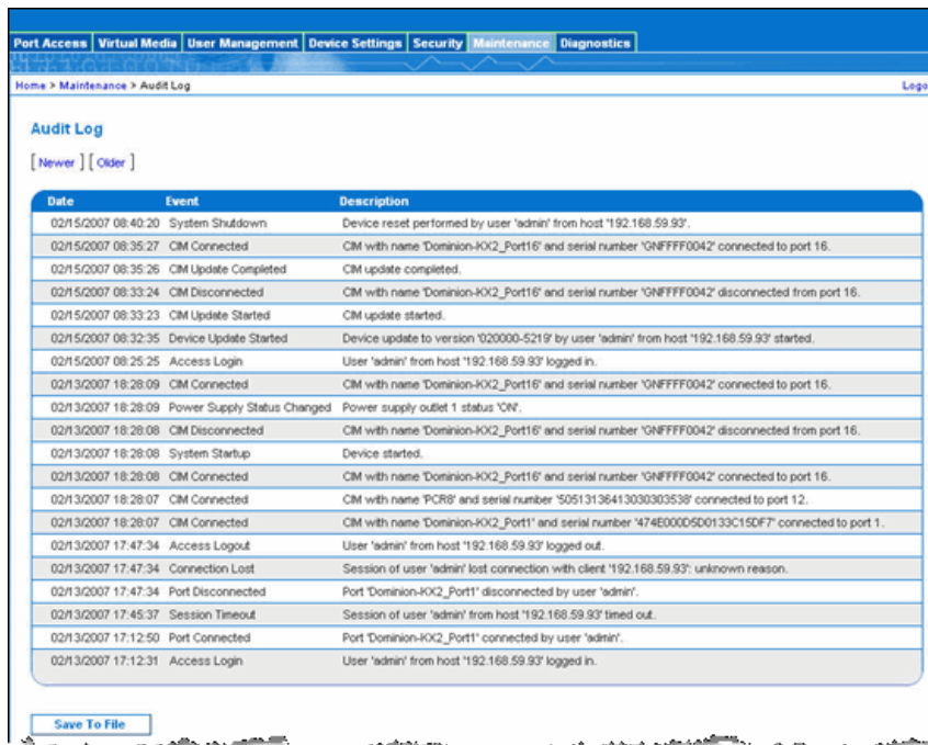
Figure 71: Audit Log
