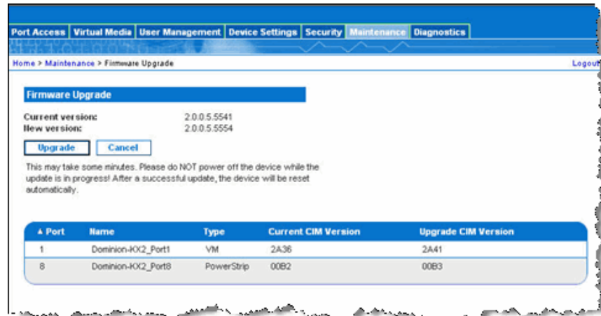
Figure 76: Firmware Upgrade Review
