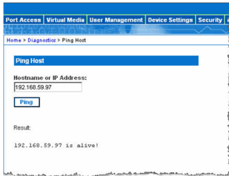
Figure 85: Ping Host
