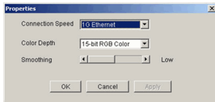
Figure 26: Properties Dialog
