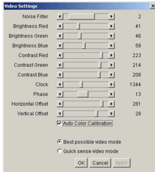
Figure 32: Video Settings
