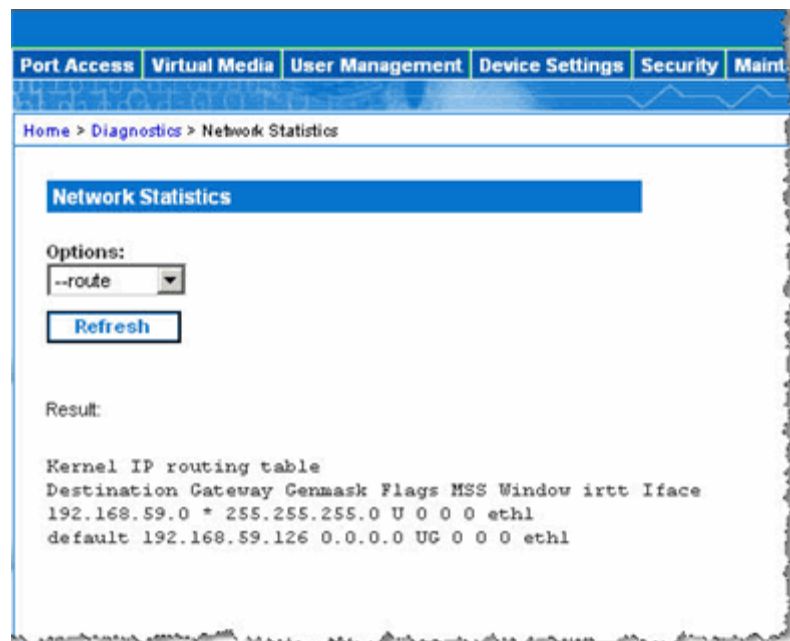
Figure 84: Network Statistics (route)
