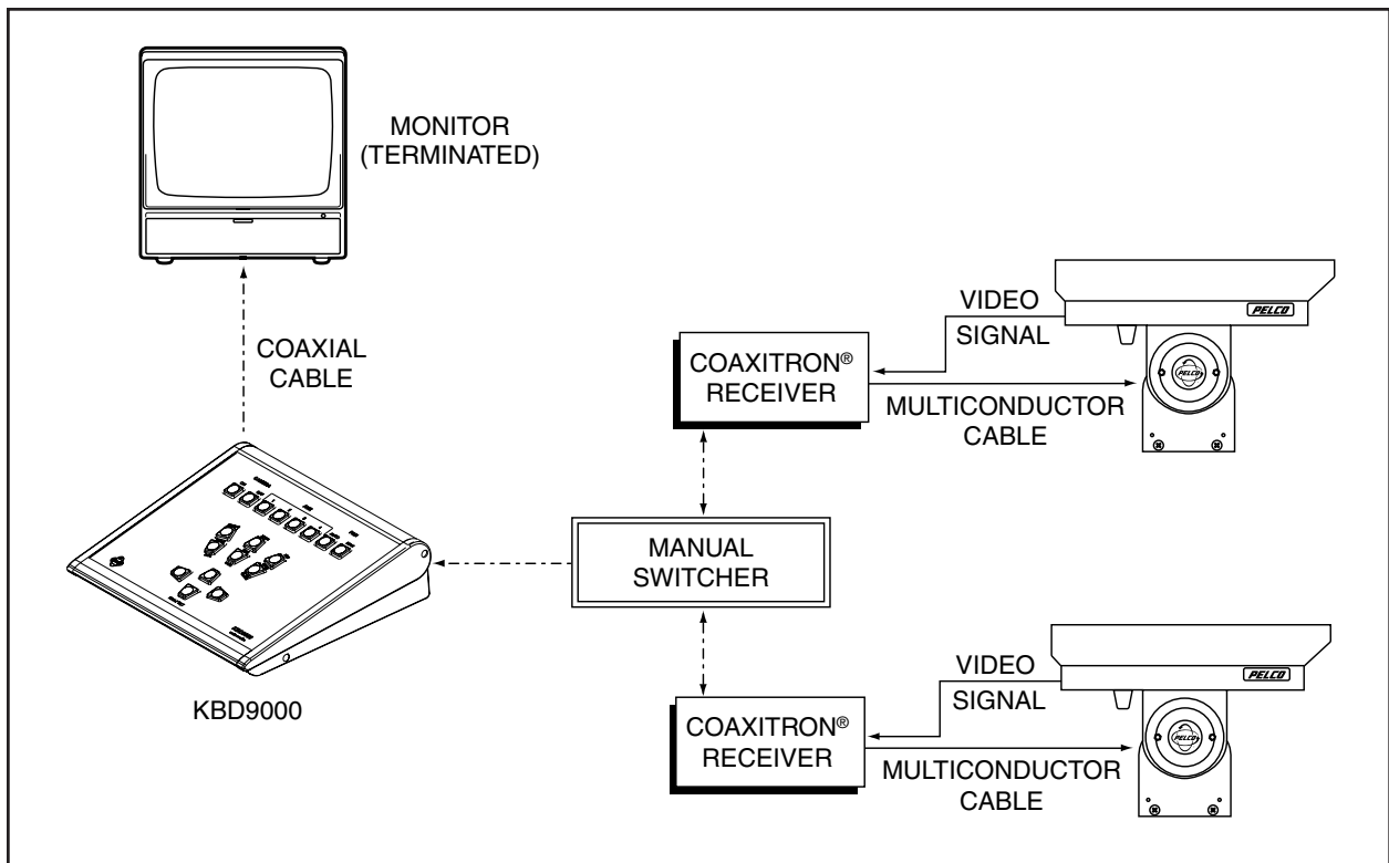
Figure 2. KBD9000 Configuration with Manual Video Switcher and Multiple Cameras
