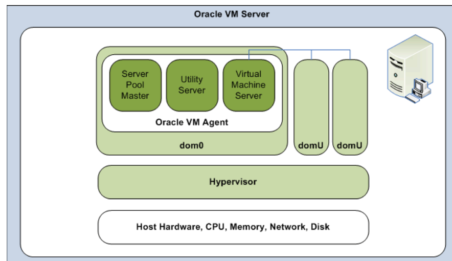
Figure D-1 Oracle VM Agent
