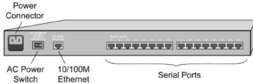
Figure 1-3. 16-Port NPort Server Pro Rear Panel (DE-303)
