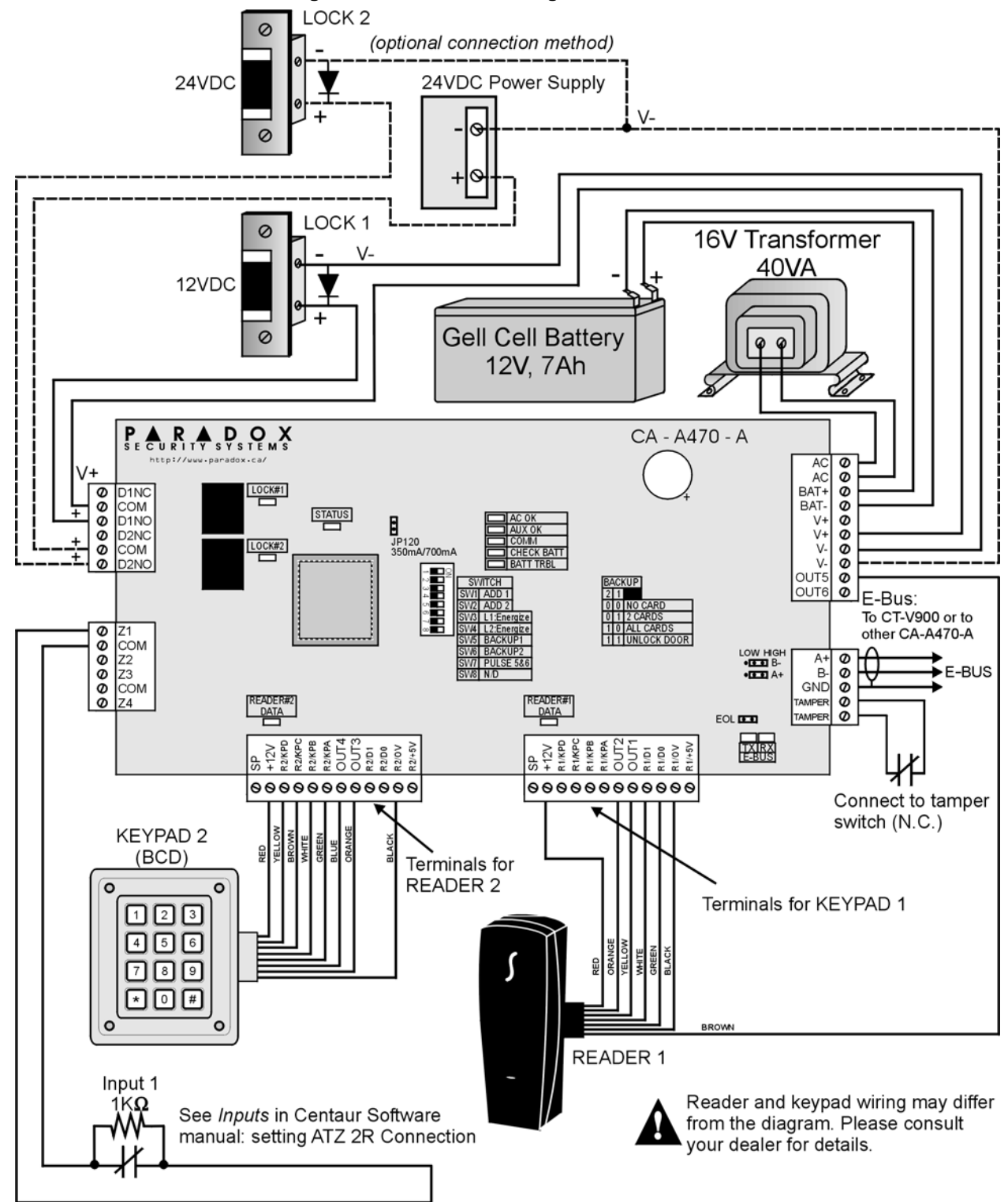
Figure 6: Connection drawing of the CA-A470-A
