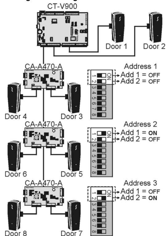
Figure 1: Setting the network address
