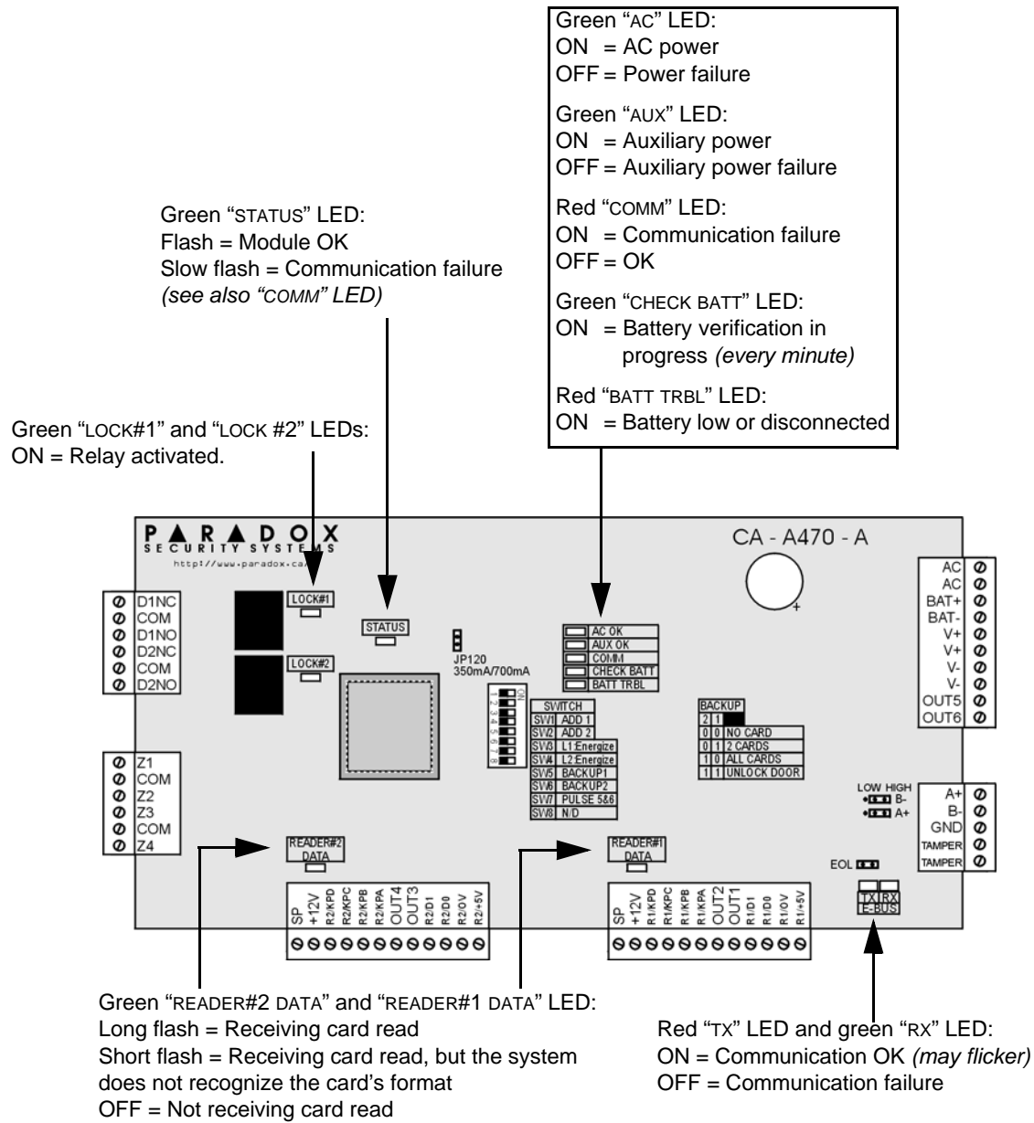
Figure 5: CA-A470-A indicators
