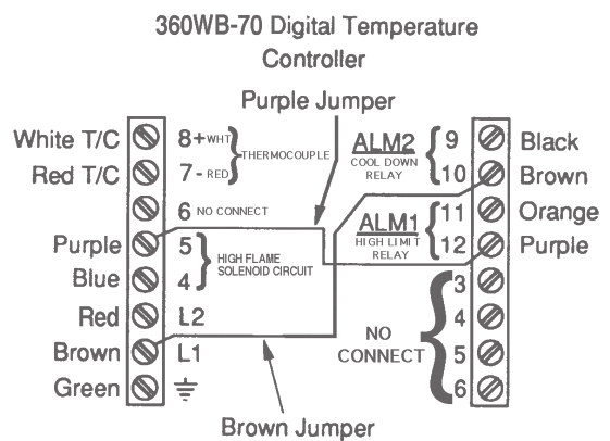
Figure 10 - Wiring Diagram Showing Electrical Connections (Refer to Table 2)
