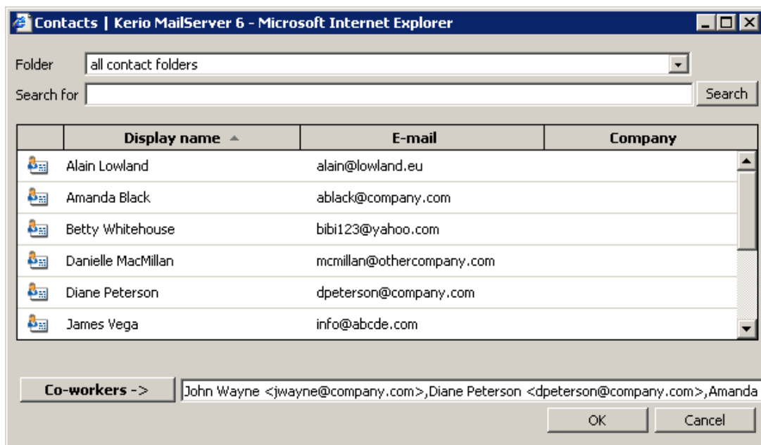
Figure 1.84 Select
