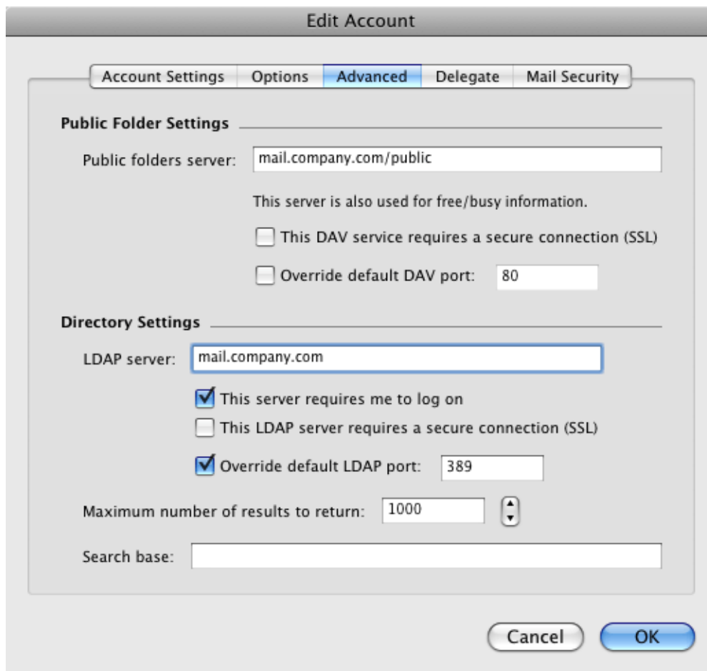
Figure 10.12 Advanced
