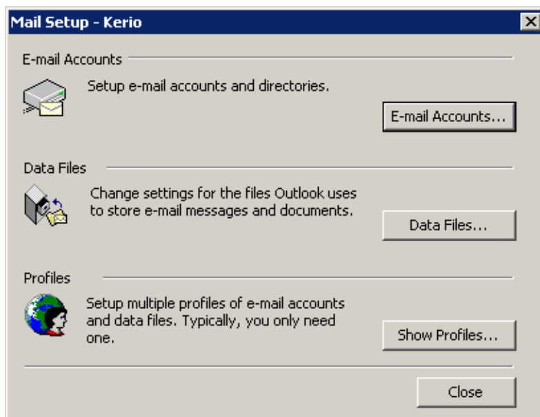
Figure 5.1 Profile setup
