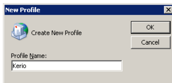
Figure 5.3 New profile
