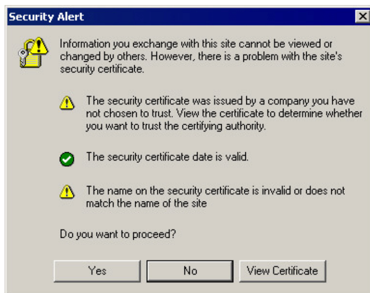
Figure 7.6 Security Alert
