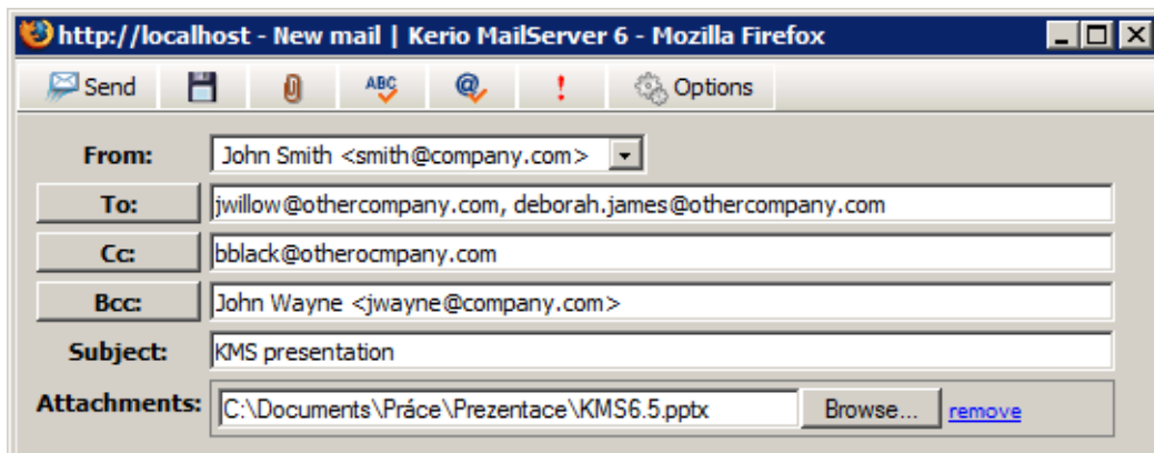
Figure 1.30 E-mail header
