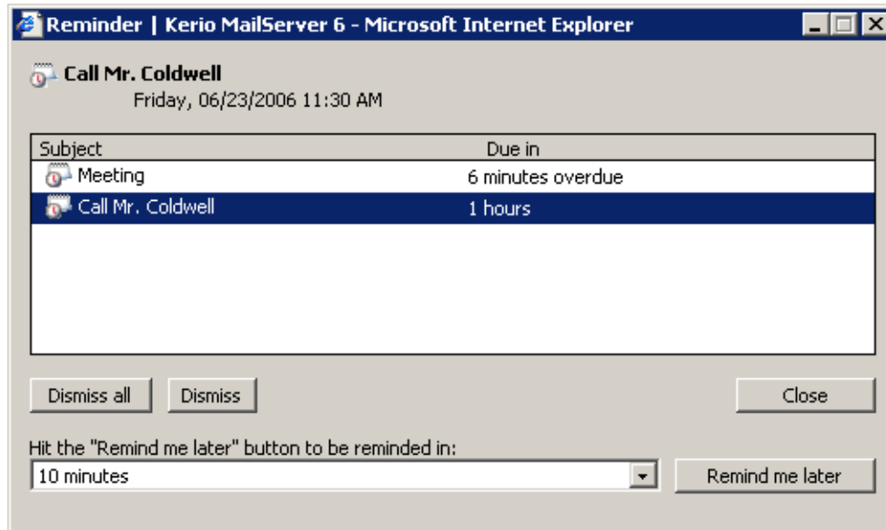
Figure 1.67 Reminder
