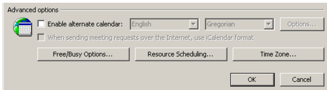
Figure 5.40 Calendar Options
