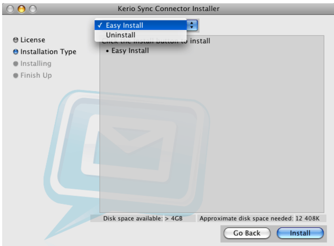
Figure 13.2 Installation settings
