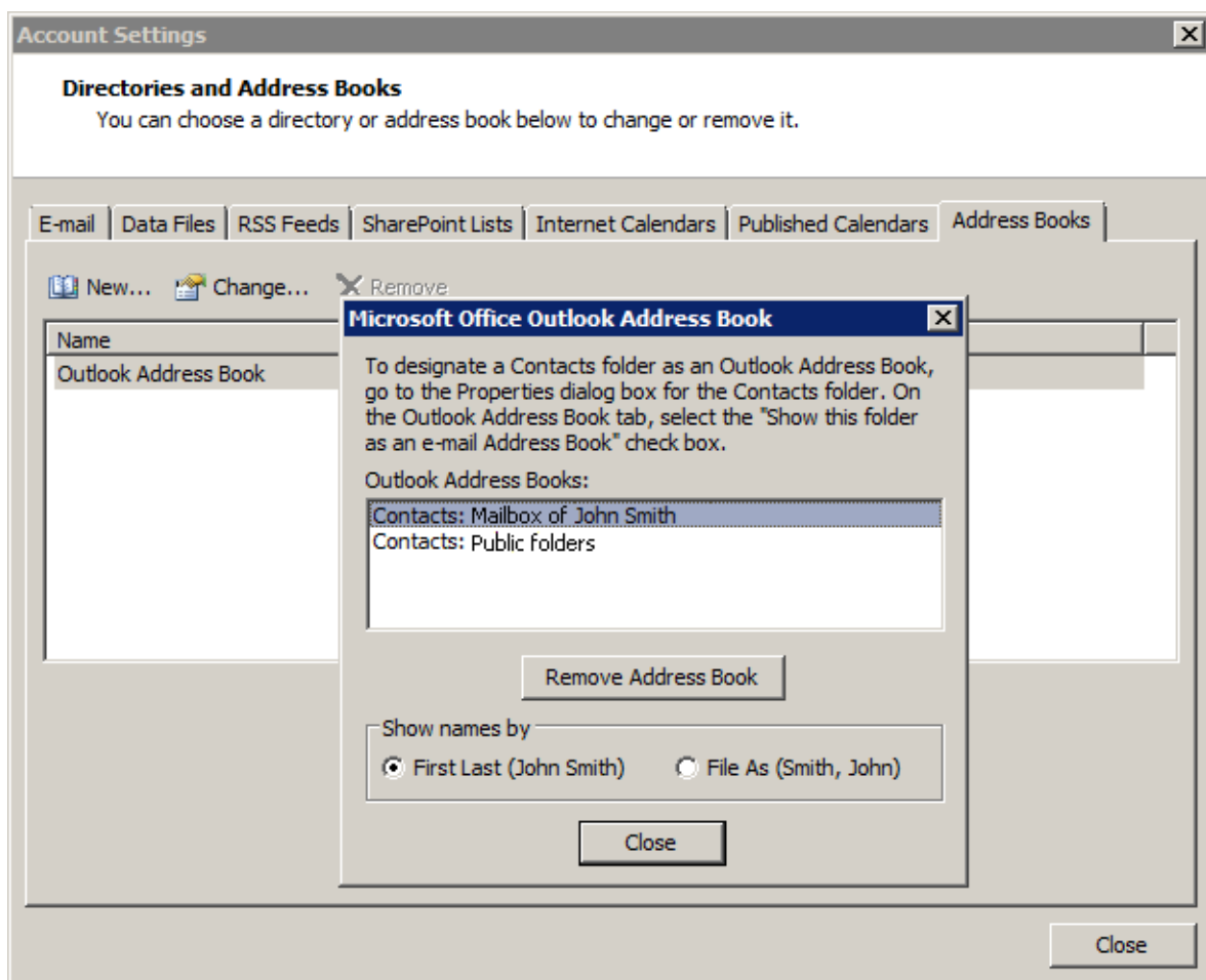
Figure 6.5 Address Book
