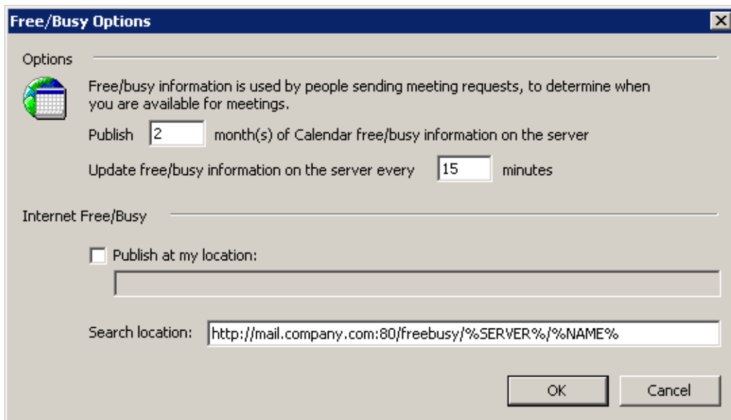
Figure 5.41 Free/Busy options
