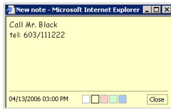
Figure 1.92 Note
