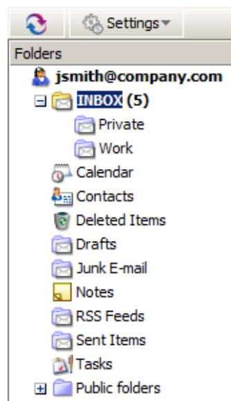
Figure 1.9 Folder tree
