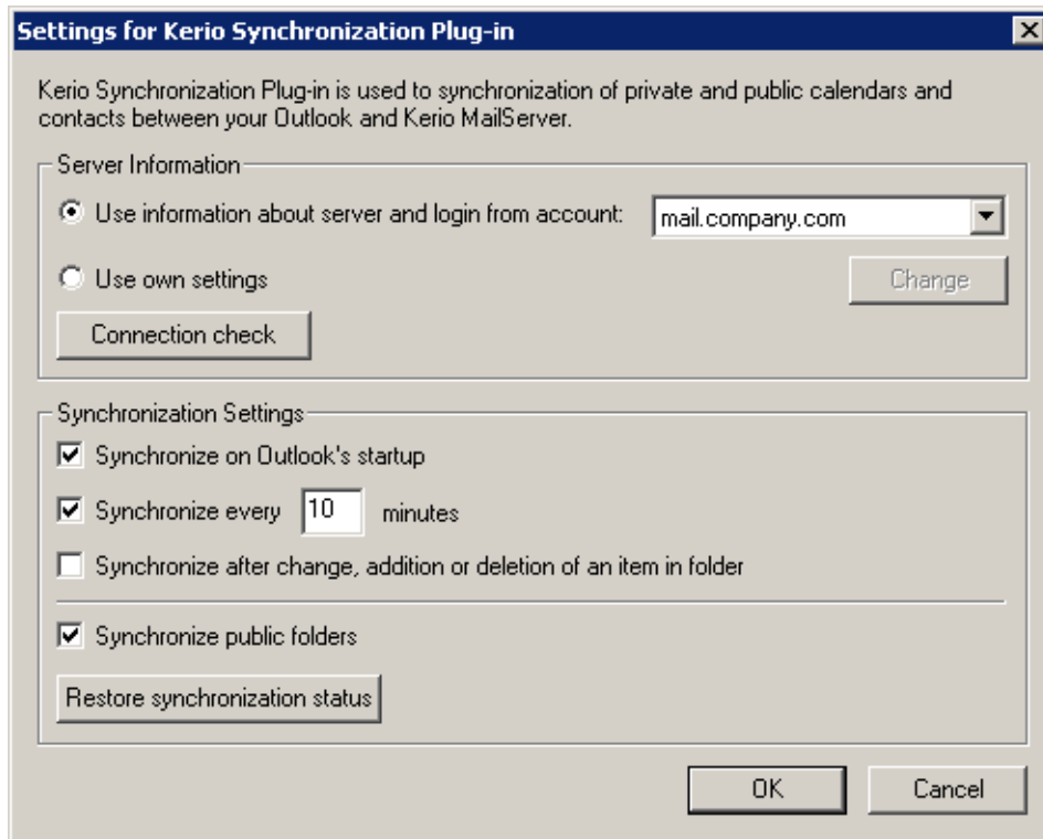
Figure 7.3 Synchronization settings
