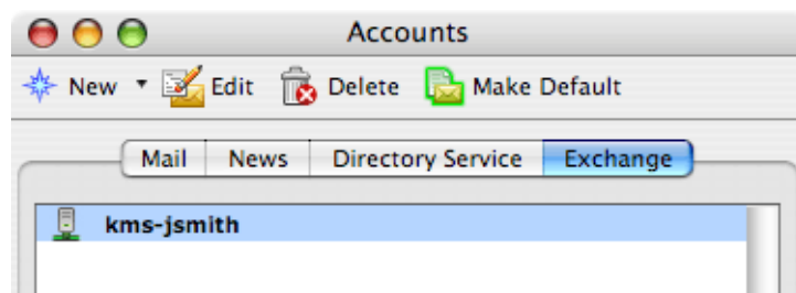
Figure 10.7 Accounts
