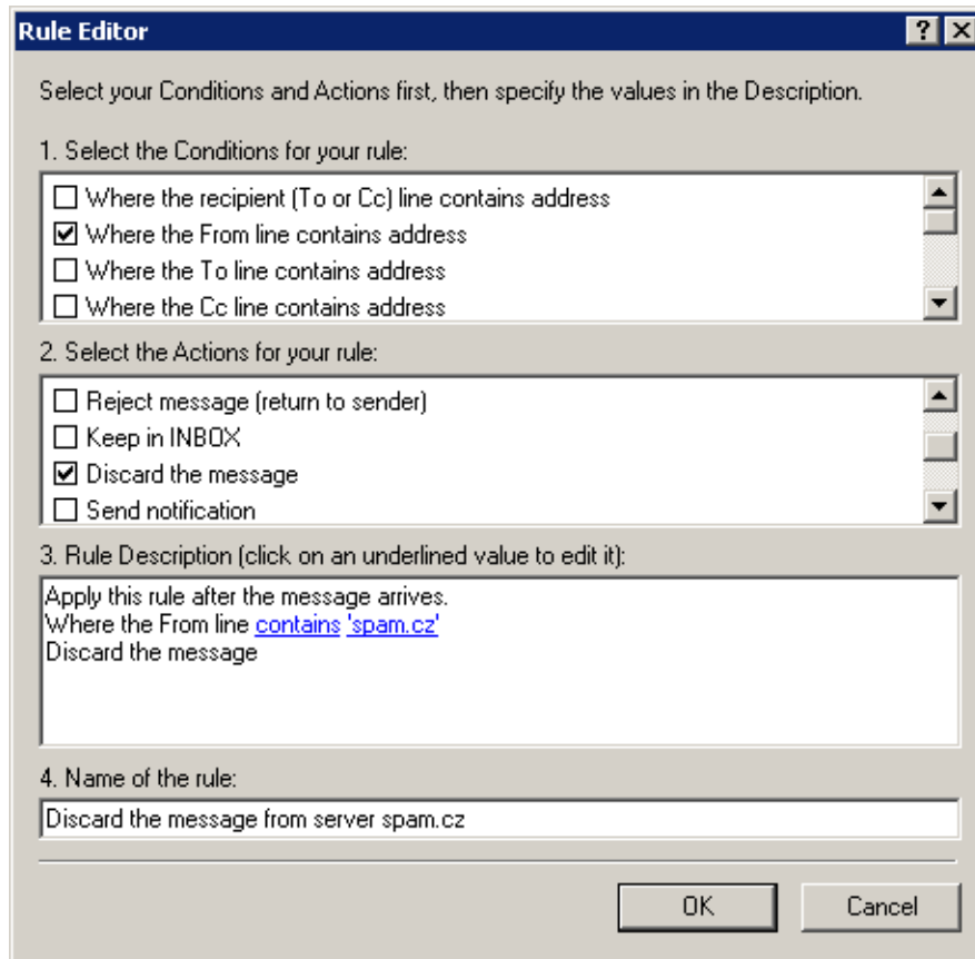
Figure 5.20 Rule Editor
