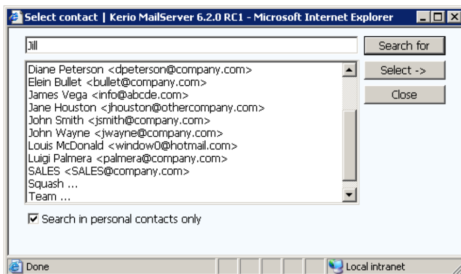
Figure 2.16 Select
