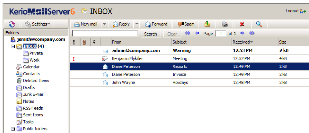
Figure 1.10 Email
