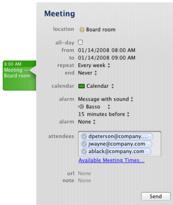
Figure 11.10 Meeting settings
