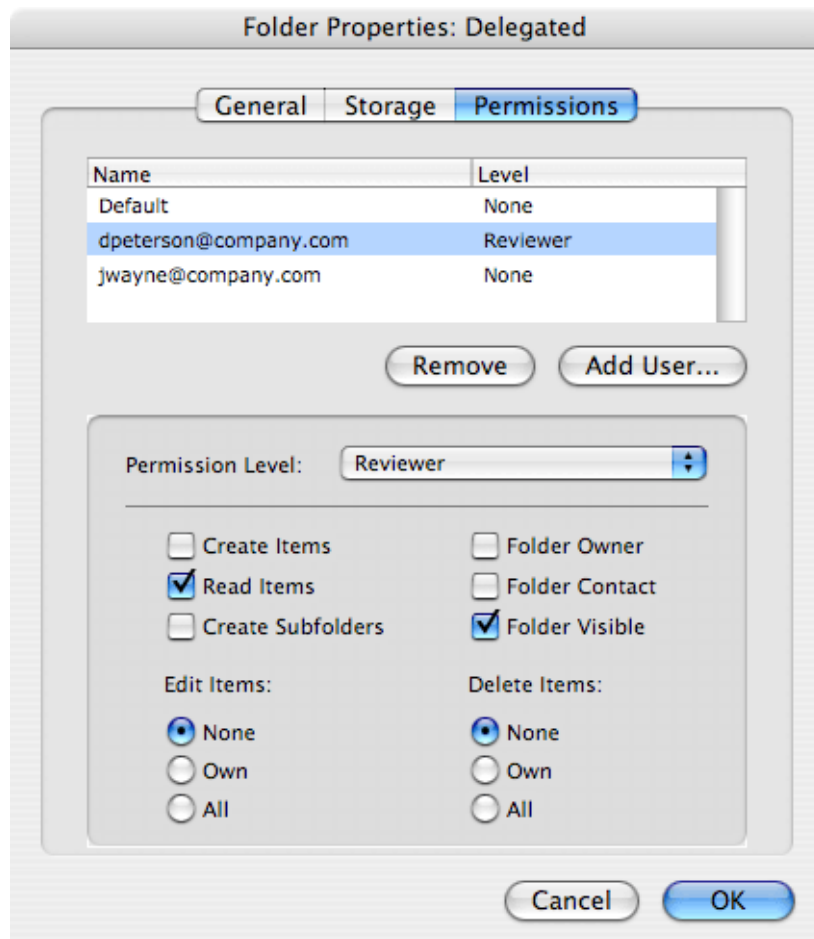
Figure 10.17 Sharing folders
