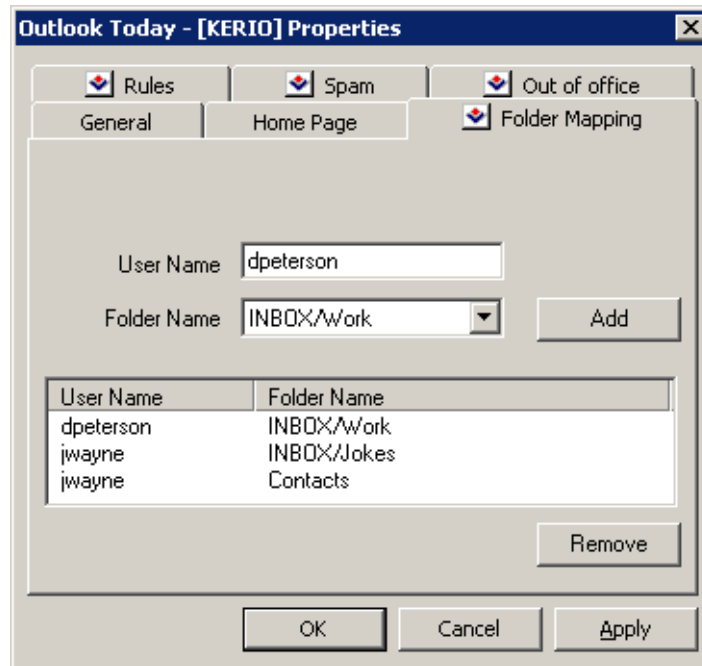
Figure 5.17 Folder mapping
