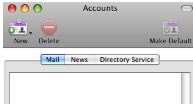
Figure 10.10 Accounts
