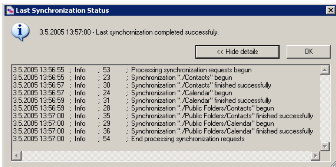
Figure 7.5 Synchronization status
