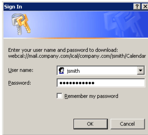
Figure 8.5 User authentication
