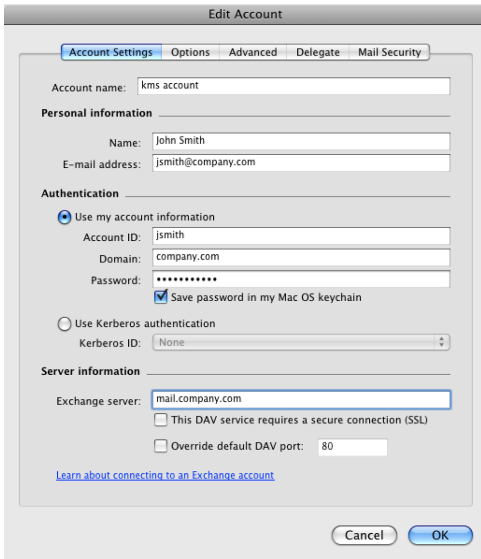
Figure 10.11 Account Settings
