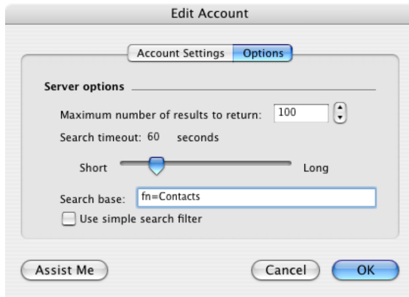
Figure 10.14 LDAP settings
