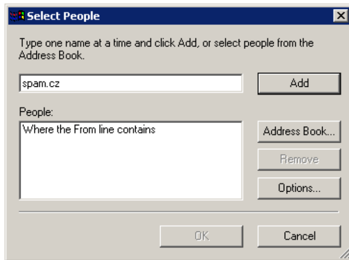
Figure 6.19 Select People
