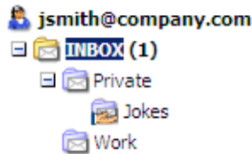
Figure 1.111 Shared folder
