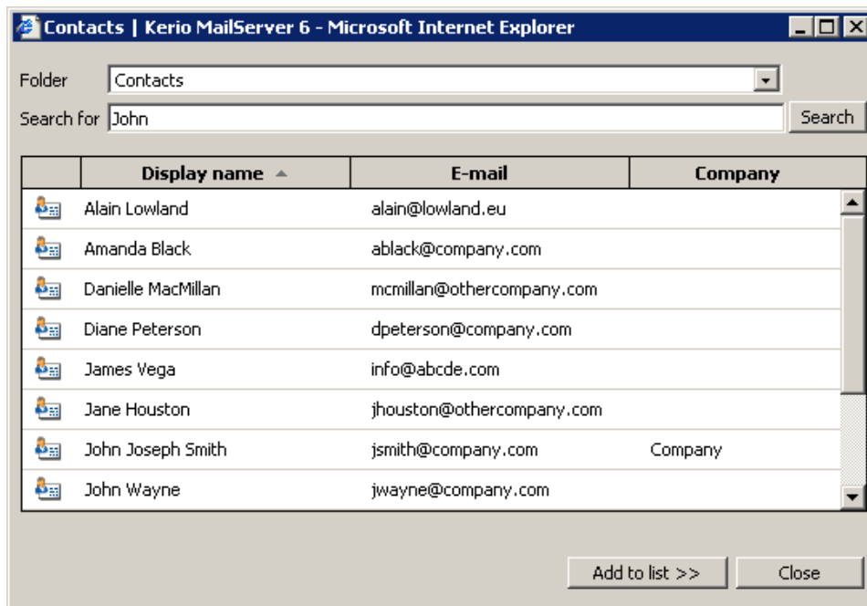
Figure 1.59 Select
