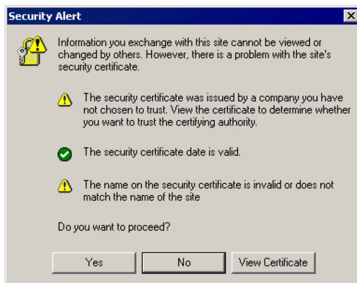
Figure 6.14 Security Alert
