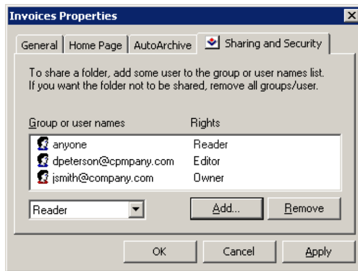
Figure 5.15 Folder Sharing
