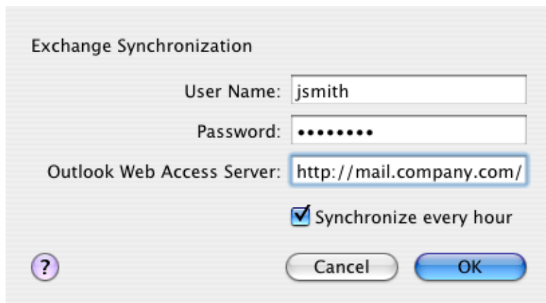
Figure 12.3 Synchronization setup
