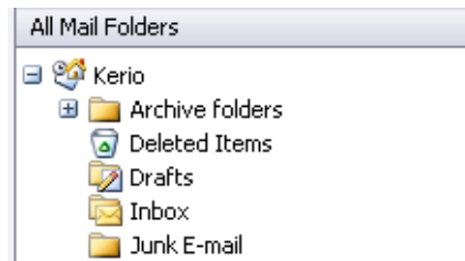
Figure 5.18 Archive folders
