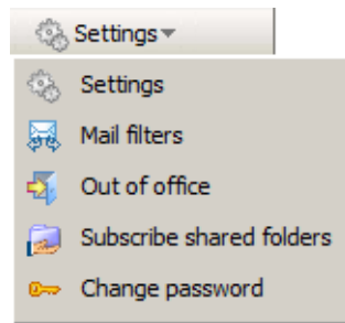
Figure 1.131 Settings Menu
