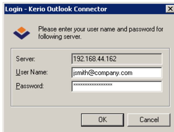
Figure 5.14 Login dialog
