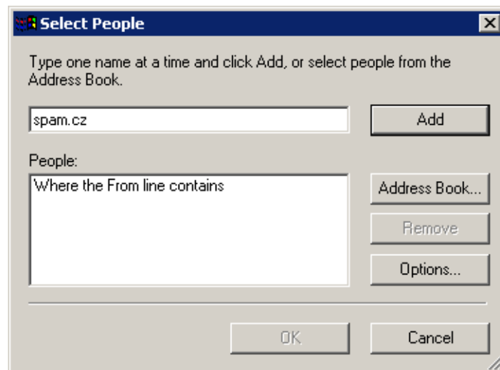
Figure 5.21 Select People
