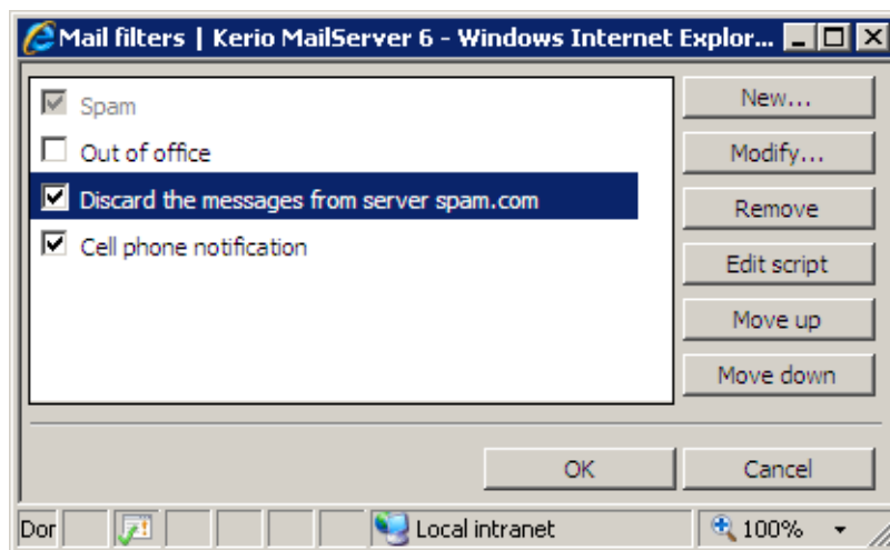
Figure 1.132 Rule list
