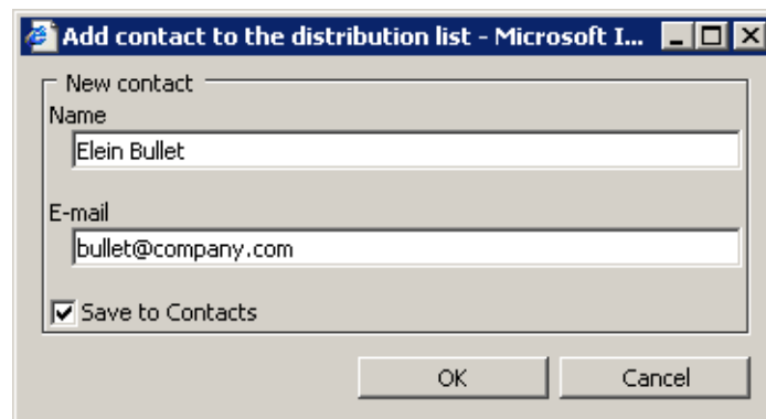
Figure 1.60 Add
