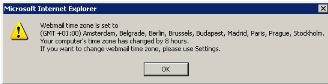
Figure 1.117 Warning
