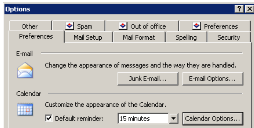
Figure 5.39 Preferences
