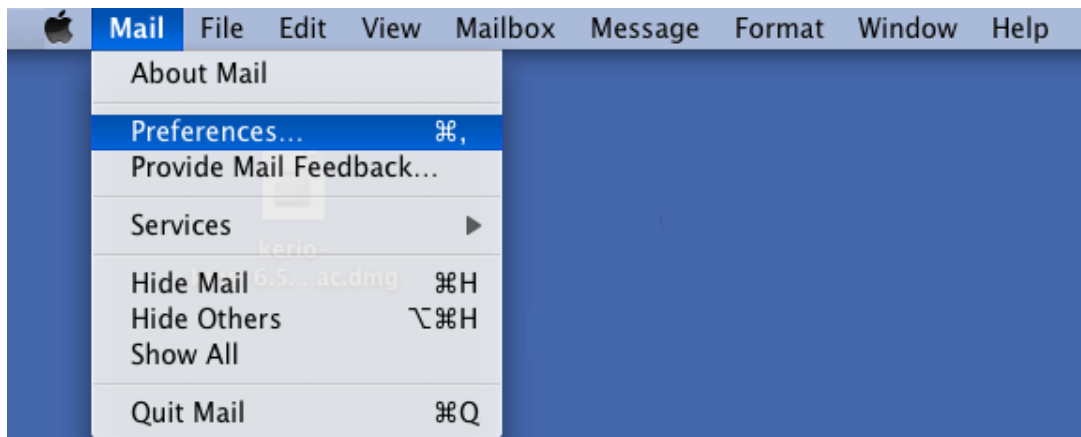
Figure 14.1 Mail → Preferences
