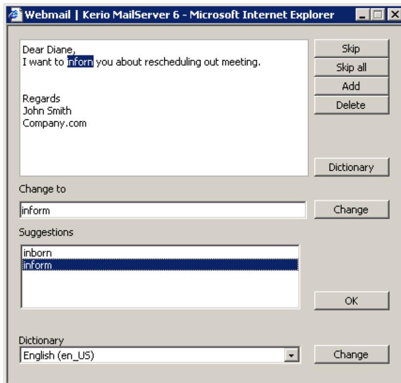
Figure 1.36 Spellchecker
