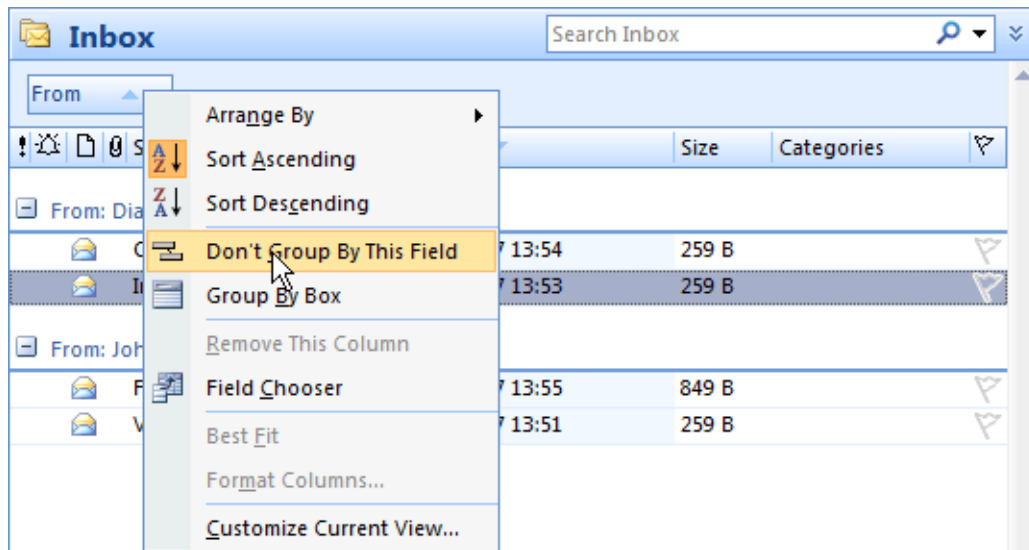
Figure 6.26 Grouping removal
