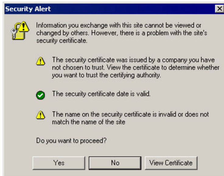
Figure 5.36 Security Alert
