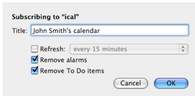
Figure 11.4 Setting details
