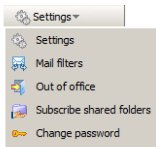
Figure 1.129 Settings Menu
