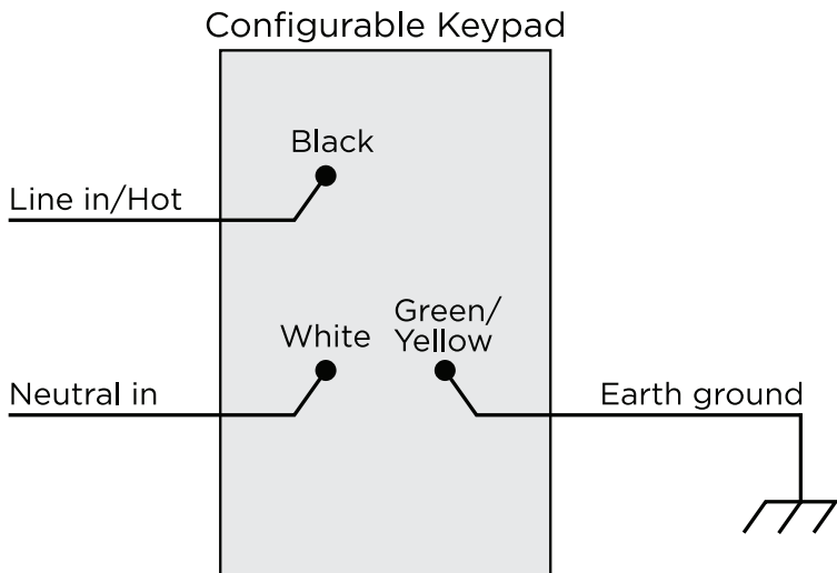
Figure 2. Keypad wiring
