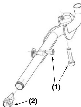
(1) Bolt (2) Spark arrester
